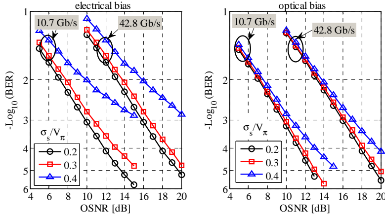
Fig.5: Receiver sensitivity after 8x80km spans of SSMF transmission with electrical biasing (left) and optical biasing (right).
